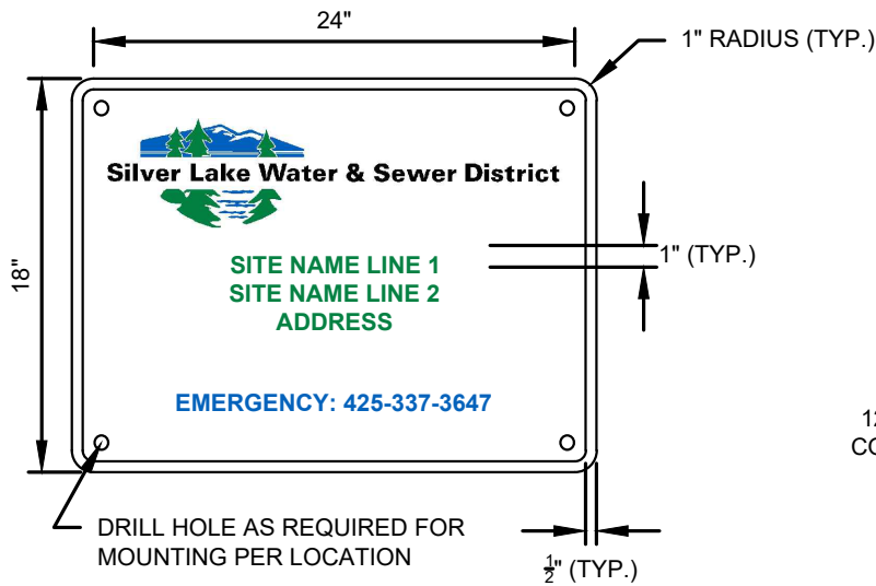
TYPICAL SITE SIGN
