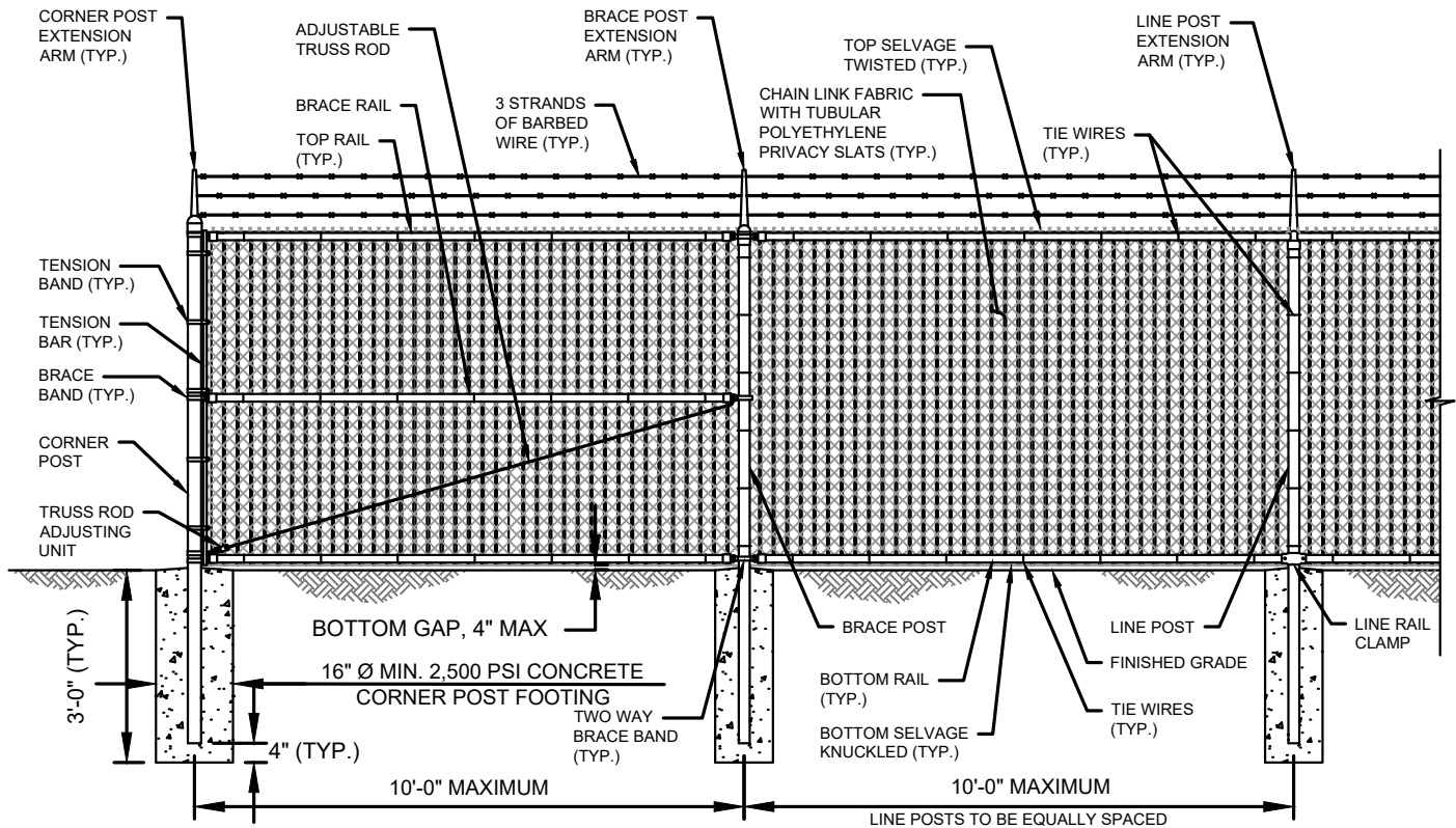
ELEVATION VIEW FROM SITE INTERIOR
