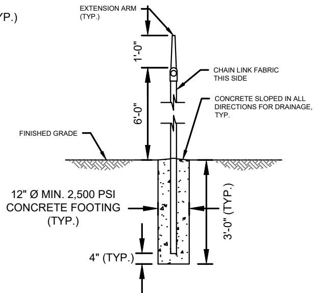
LINE/BRACE POST SECTION
