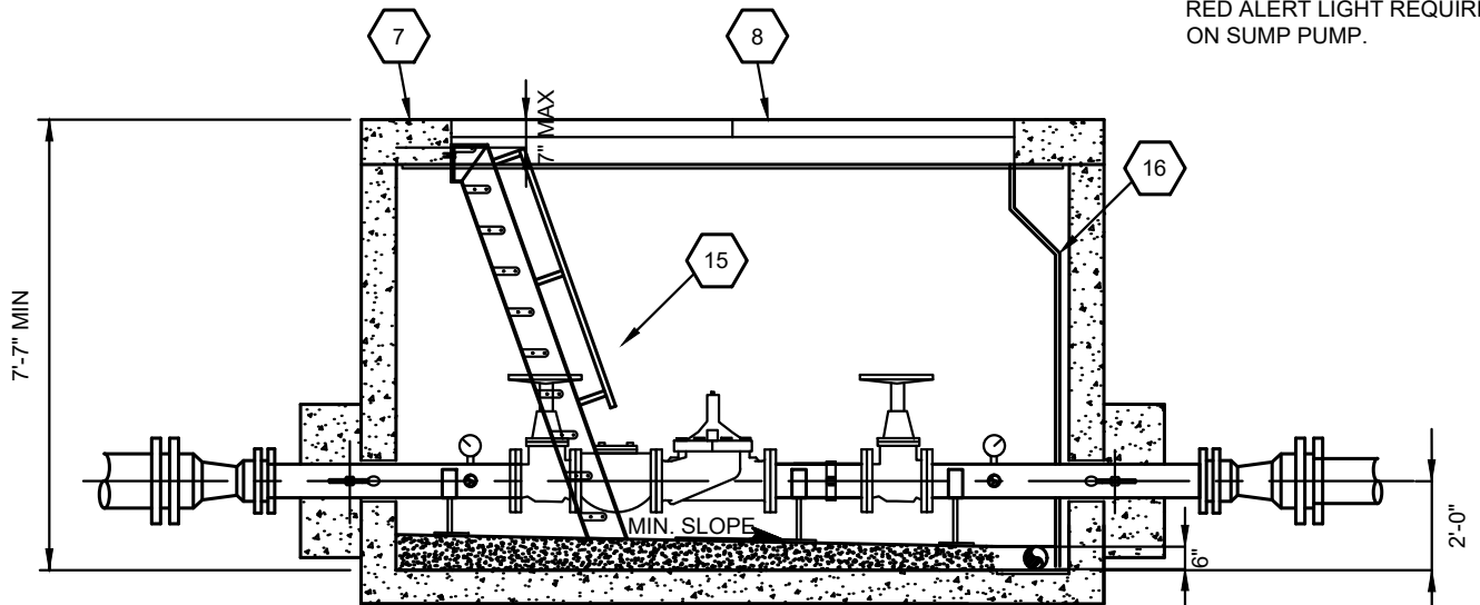
A SECTION
